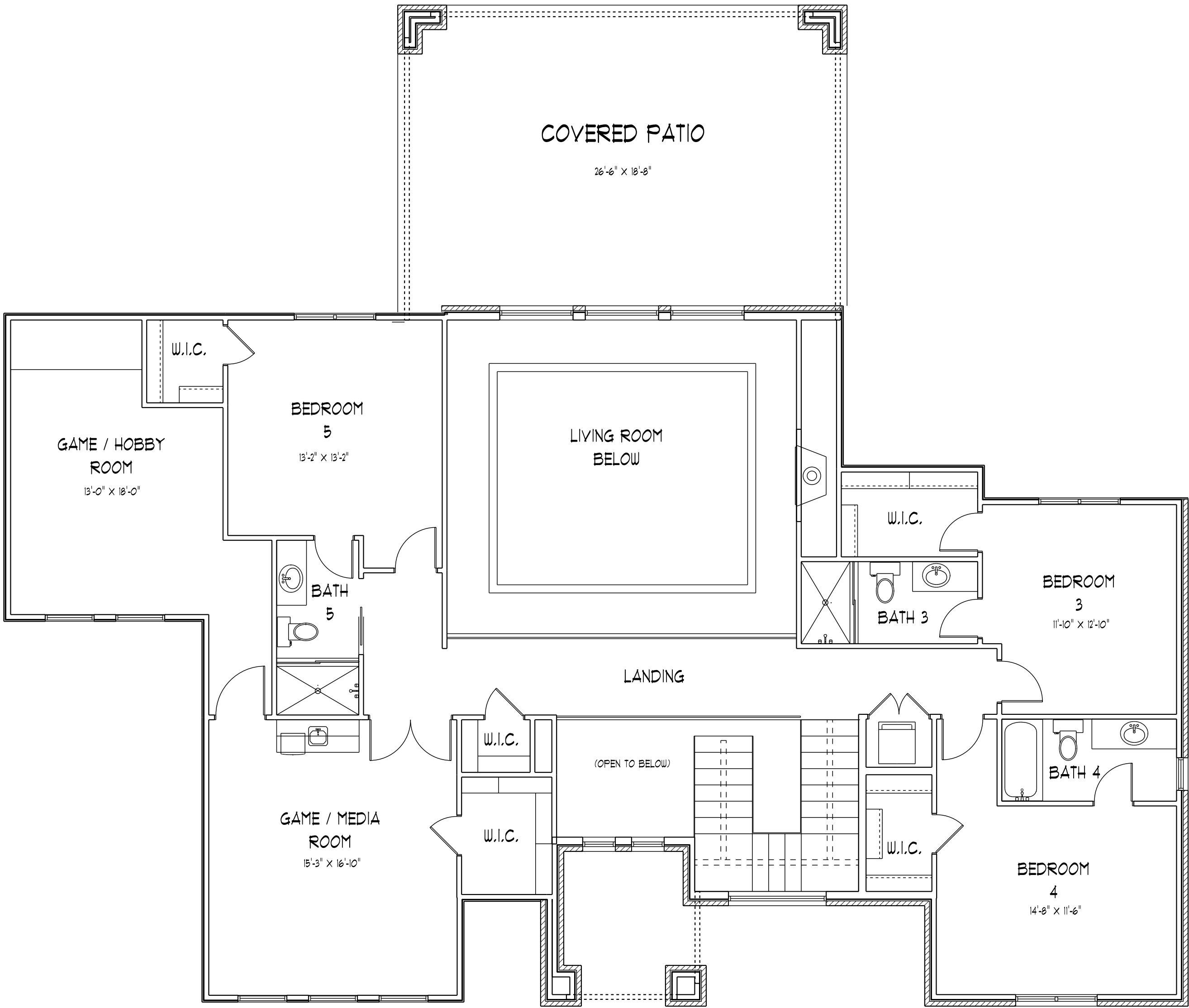
2nd FLOOR
